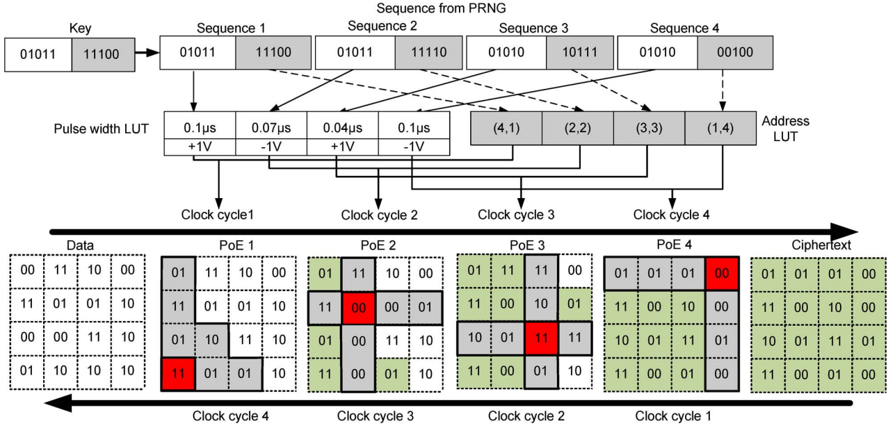
Fig. 18. SNVMM operation: Encryption/Decryption in a 4 \times 4 crossbar. The component in red shows the PoE, grey the affected memristors, and green the memristors whose contents are encrypted [73].
